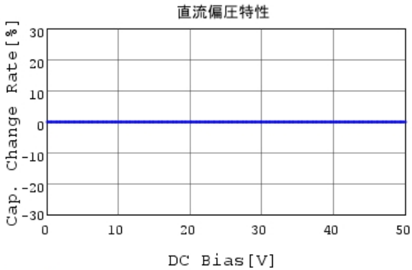
GCQ1555C1H270FB01 C-DC bias capchange, 25.0c
