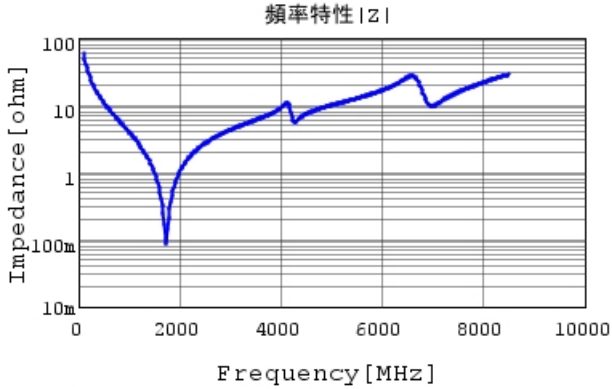
GCQ1555C1H270FB01 |Z| DCOV,25degC
