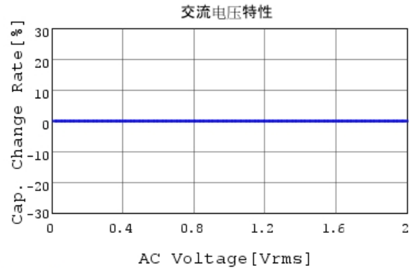
GCQ1555C1H270FB01 C-AC Voltage capchange, DC
