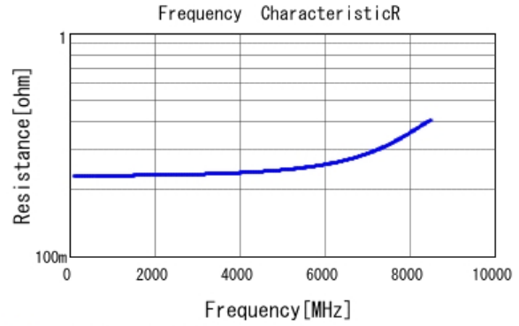
■ GCQ1555C1H1R3WB01 R DC0V, 25degC
