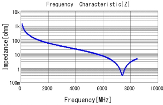
■ GCQ1555C1H1R3WB01 |Z| DC0V, 25degC
