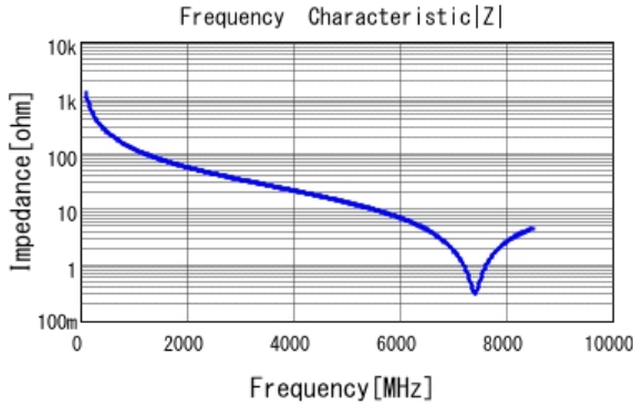
■ GCQ1555C1H1R3BB01 |Z| DC0V, 25degC
