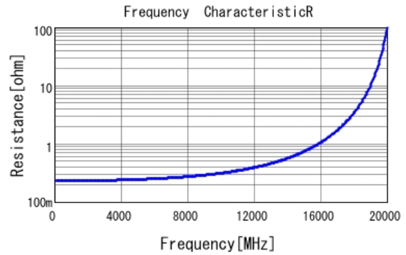
■ GCQ1555C1H1R0BB01 R DC0V, 25degC
