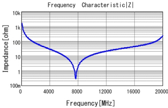
■ GCQ1555C1H1R0BB01 |Z| DC0V, 25degC
