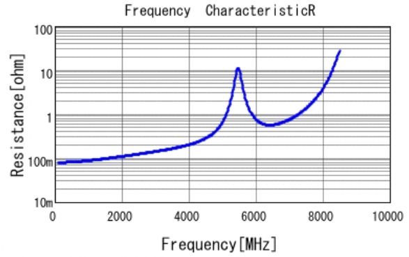
■ GCQ1555C1H150JB01 R DC0V, 25degC
