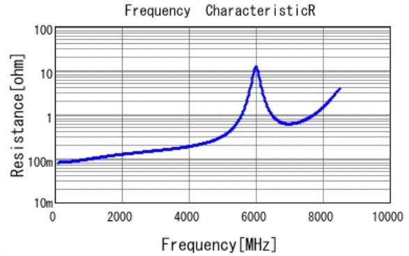
■ GCQ1555C1H120JB01 R DC0V, 25degC
