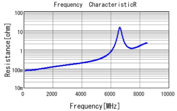
■ GCQ1555C1H100JB01 R DC0V, 25degC
