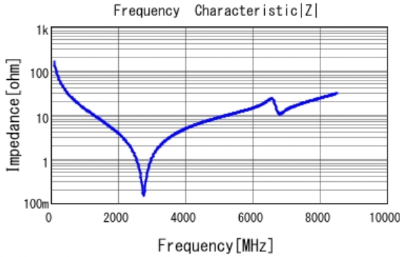
■ GCQ1555C1H100JB01 |Z| DC0V, 25degC
