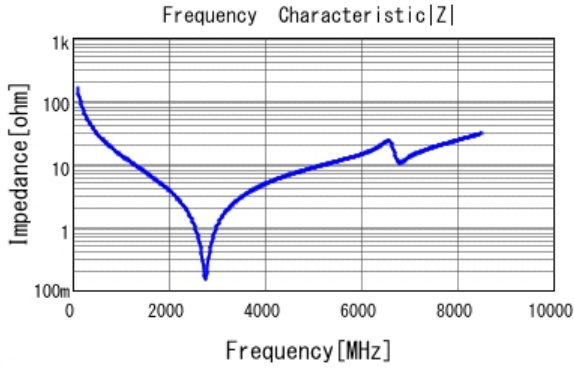
■ GCQ1555C1H100FB01 |Z| DC0V, 25degC
