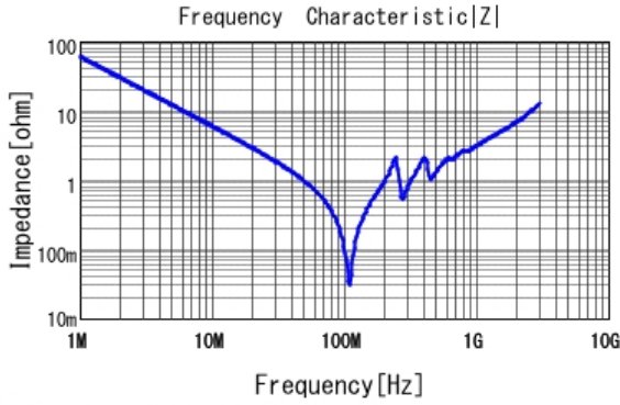
GCM43Q7U3A272JX01 |Z| DC0V, 25degC
