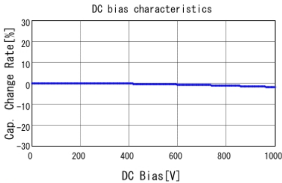
GCM43Q7U3A272JX01 C-DC bias capchange, 25.0degC, AC1V
