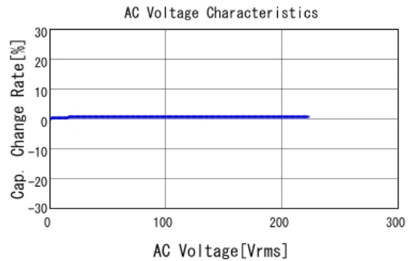
■ GCM32Q7U2J682JX01 C-AC Voltage capchange, DC0V, 25.0d
