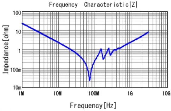
■ GCM32Q7U2J682JX01 |Z| DC0V, 25degC
