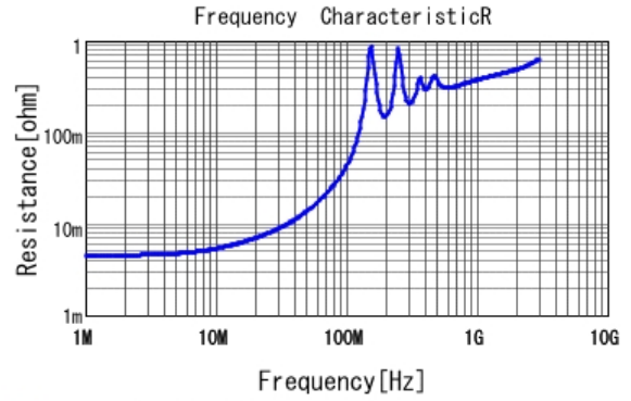
■ GCM32Q7U2J682JX01 R DC0V, 25degC
