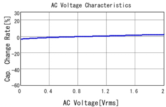
■ GCM32ER71H105KA37 C-AC Voltage capchange, DCOV, 25.0d
