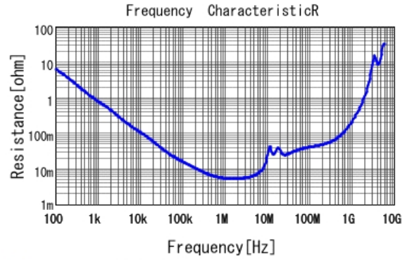
■ GCM32ER71H105KA37 R DCOV, 25degC
