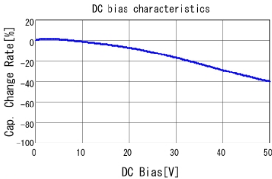
■ GCM32ER71H105KA37 C-DC bias capchange, 25.0degC, AC1.
