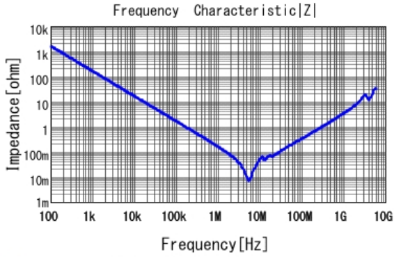
■ GCM32ER71H105KA37 |Z| DCOV, 25degC
