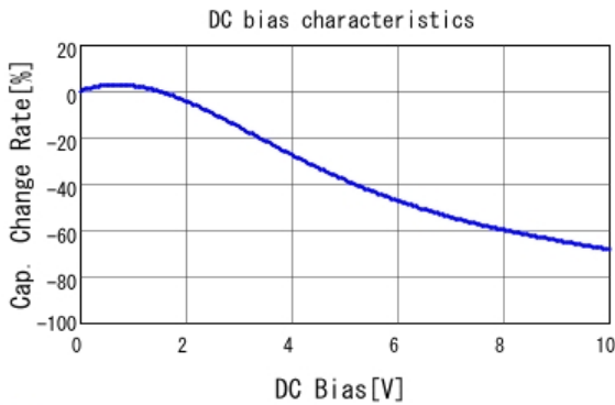
GCM32EC71A476KE02 C-DC bias capchange, 25.0degC, AC0.
