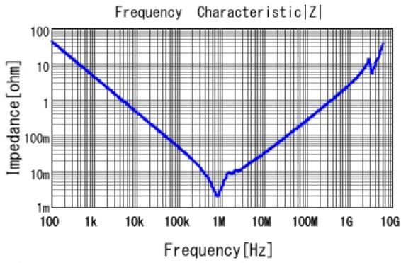
GCM32EC71A476KE02 |Z| DC0V, 25degC
