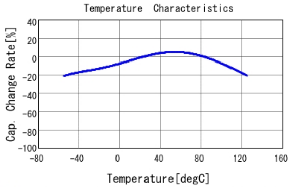
■ GCM32EC71A476KE02 C-Temp. capchange, DC0.0V, AC0.25Vr
