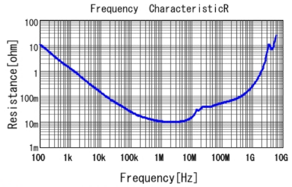
GCM31MR71H684KA55 R DCOV, 25degC
