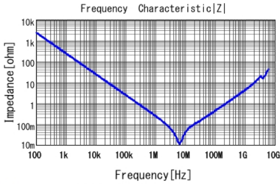
GCM31MR71H684KA55 |Z| DCOV, 25degC
