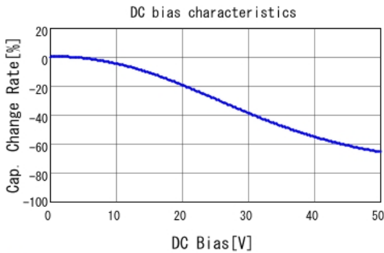
GCM31MR71H684KA55 C-DC bias capchange, 25.0degC, AC1.
