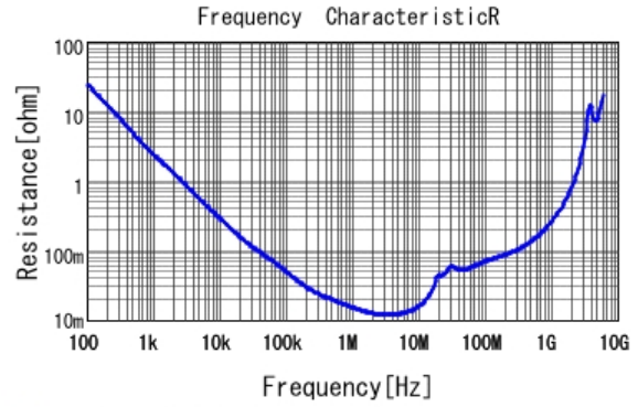
■ GCM31MR71H334KA37 R DCOV, 25degC
