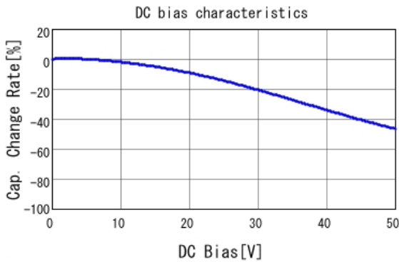
■ GCM31MR71H334KA37 C-DC bias capchange, 25.0degC, AC1.
