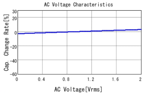
■ GCM31MR71H334KA37 C-AC Voltage capchange, DCOV, 25.0d
