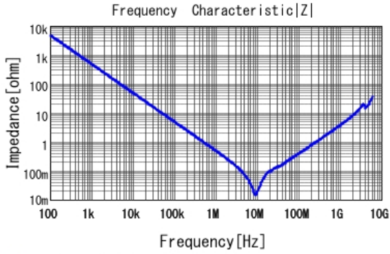
■ GCM31MR71H334KA37 |Z| DCOV, 25degC
