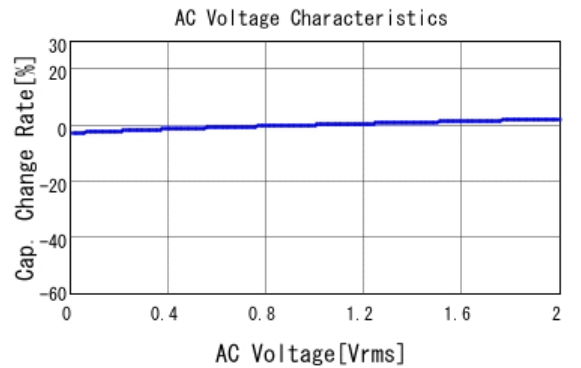
GCM31CR72A105KA03 C-AC Voltage capchange, DC0V, 25.0d
