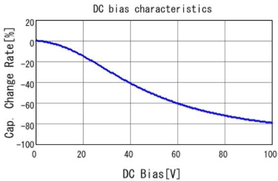
GCM31CR72A105KA03 C-DC bias capchange, 25.0degC, AC1.
