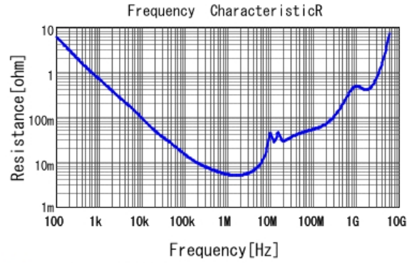
GCM31CR72A105KA03 R DC0V, 25degC
