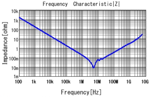
GCM31CR72A105KA03 |Z| DC0V, 25degC
