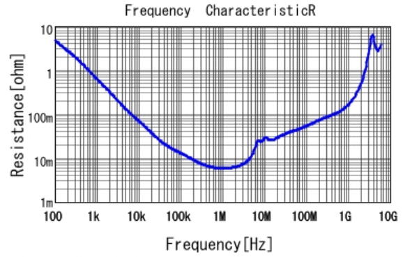
GCM31CL8EL225KE07 R DC0V, 25degC
