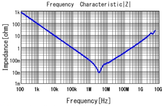
GCM31CL8EL225KE07 |Z| DC0V, 25degC
