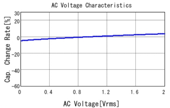
GCM31CL8EL225KE07 C-AC Voltage capchange, DC0V, 25.0d
