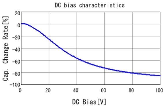
GCM31CL8EL225KE07 C-DC bias capchange, 25.0degC, AC1.
