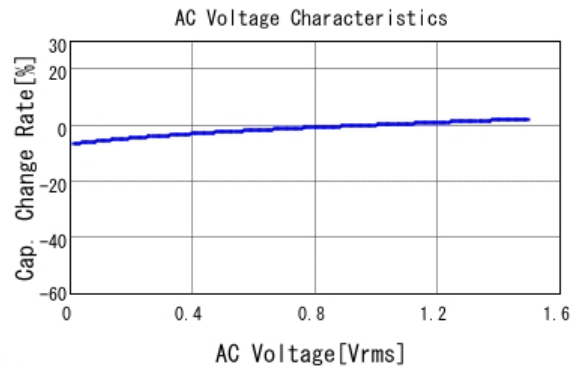
GCM31CD7YA106KE36 C-AC Voltage capchange, DCOV, 25.0d
