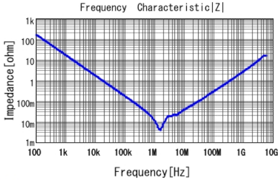
GCM31CD7YA106KE36 |Z| DCOV, 25degC
