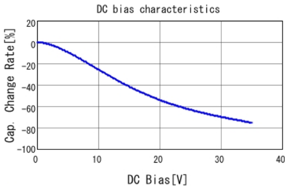
GCM31CD7YA106KE36 C-DC bias capchange, 25.0degC, AC1V
