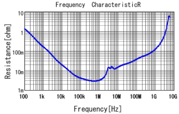
GCM31CD7YA106KE36 R DCOV, 25degC
