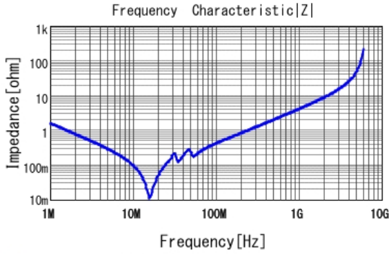
■ GCM31C5C2A104JE02 |Z| DC0V, 25degC
