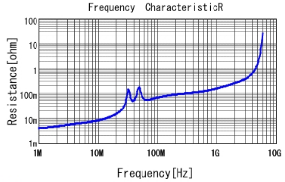
■ GCM31C5C2A104JE02 R DC0V, 25degC
