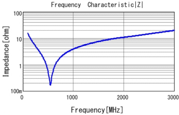
■ GCM31A7U2J101JX01 |Z| DC0V, 25degC
