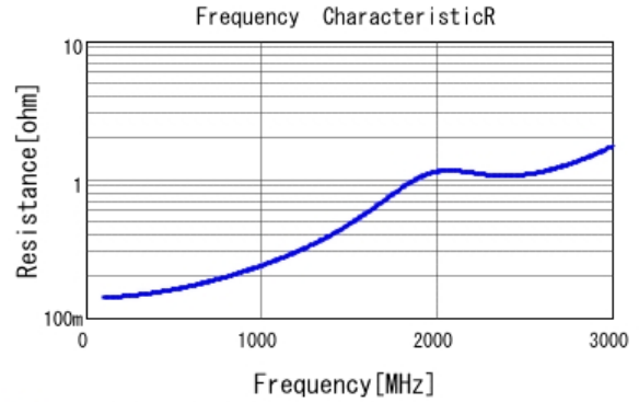
■ GCM31A7U2J101JX01 R DC0V, 25degC
