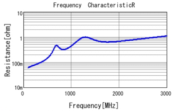
■ GCM31A5C2J681JX01 R DC0V, 25degC
