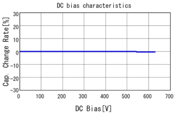
■ GCM31A5C2J681JX01 C-DC bias capchange, 25.0degC, AC1V
