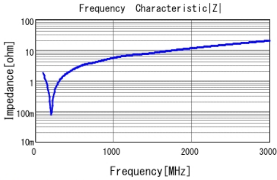
■ GCM31A5C2J681JX01 |Z| DC0V, 25degC
