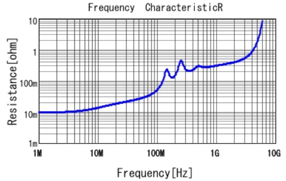
■ GCM3195C2A682JA16 R DCOV, 25degC
