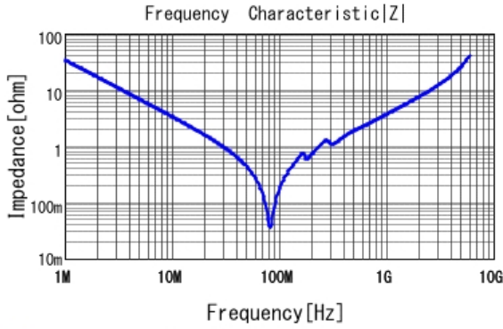
■ GCM3195C2A472JA16 |Z| DCOV, 25degC
