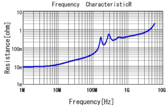
■ GCM3195C2A472JA16 R DCOV, 25degC
