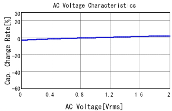
■ GCM21BR71H683KA37 C-AC Voltage capchange, DCOV, 25.0d
