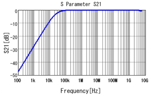
■ GCM21BR71H683KA37 S21 DC0V, 25degC
