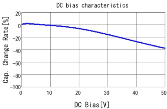
■ GCM21BR71H683KA37 C-DC bias capchange, 25.0degC, AC1.
