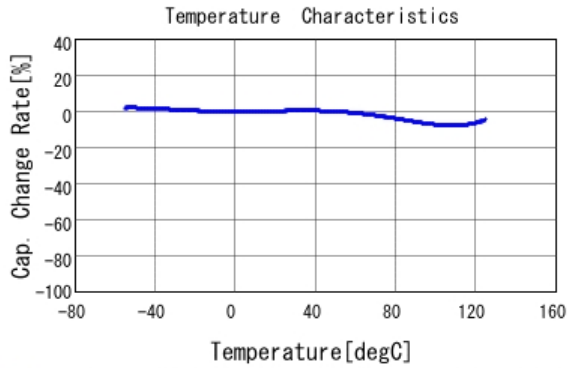
■ GCM21BR71H683KA37 C-Temp. capchange, DC0.0V, AC1.0V rm
