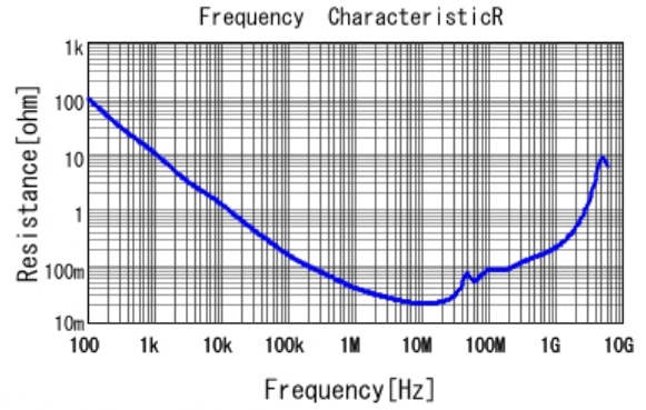
■ GCM21BR71H683KA37 R DCOV, 25degC
