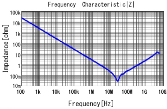
■ GCM21BR71H683KA37 |Z| DCOV, 25degC
