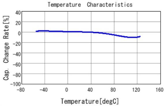
■ GCM21BR71H473KA37 C-Temp. capchange, DC0.0V, AC1.0Vrm
