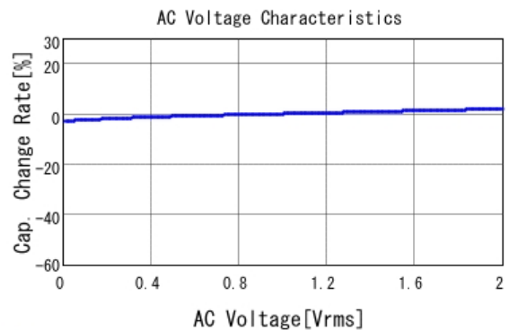
GCM21BR71H473KA37 C-AC Voltage capchange, DCOV, 25.0d
