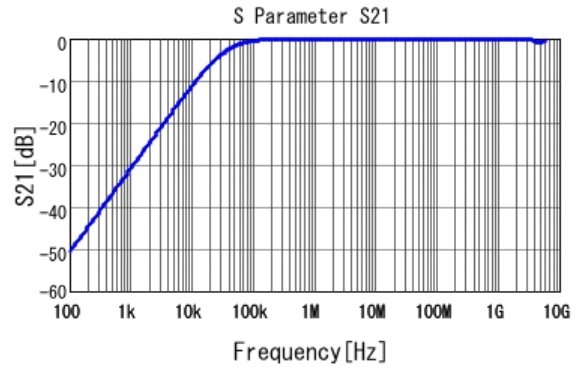
■ GCM21BR71H473KA37 S21 DC0V, 25degC
