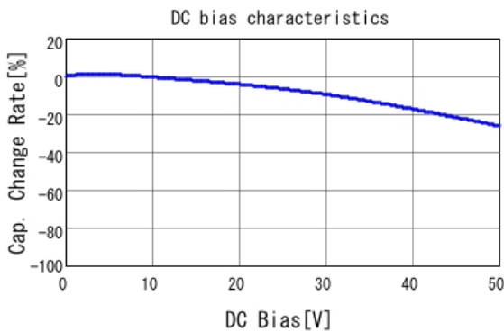
GCM21BR71H473KA37 C-DC bias capchange, 25.0degC, AC1.
