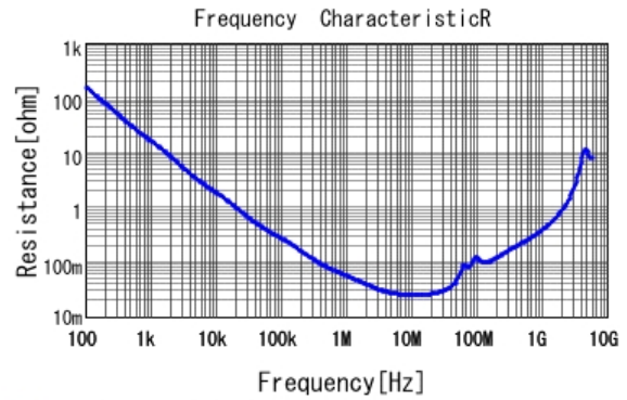
GCM21BR71H473KA37 R DCOV, 25degC
