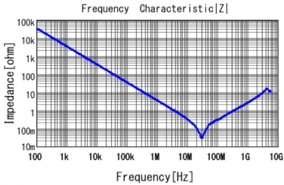
GCM21BR71H473KA37 |Z| DCOV, 25degC
