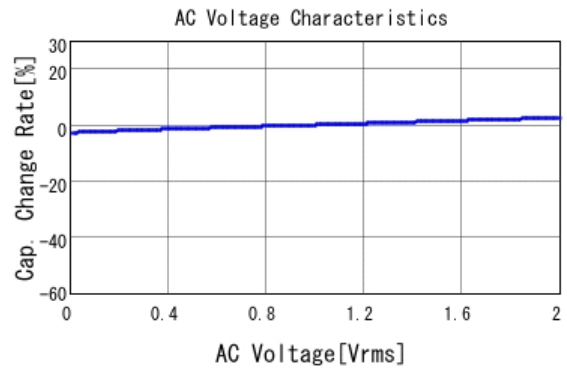
GCM21BR71E224KA37 C-AC Voltage capchange, DC0V, 25.0d
