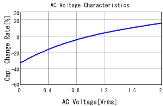
■ GCM21BR71E155KA54 C-AC Voltage capchange, DC0V, 25.0d
