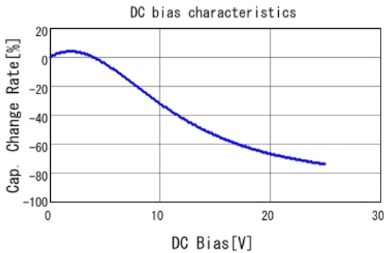
■ GCM21BR71E155KA54 C-DC bias capchange, 25.0degC, AC1.
