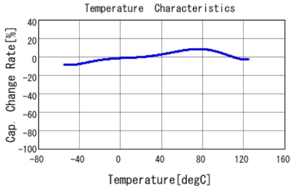
■ GCM21BR71E155KA54 C-Temp. capchange, DC0.0V, AC1.0V rm
