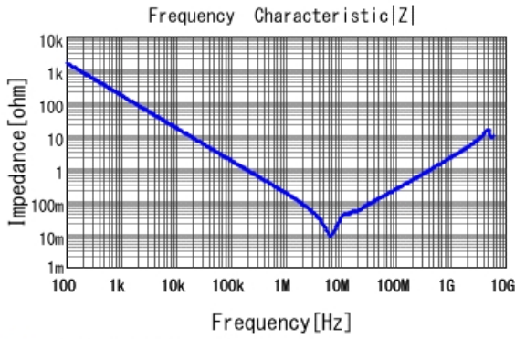
■ GCM21BR71E155KA54 |Z| DC0V, 25degC
