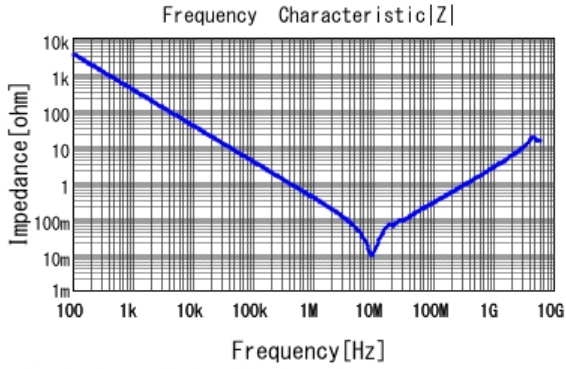
■ GCM21BR71C474KA37 |Z| DC0V, 25degC
