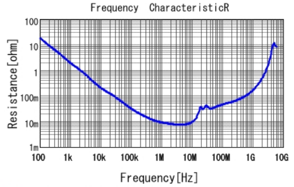
■ GCM21BR71C474KA37 R DC0V, 25degC
