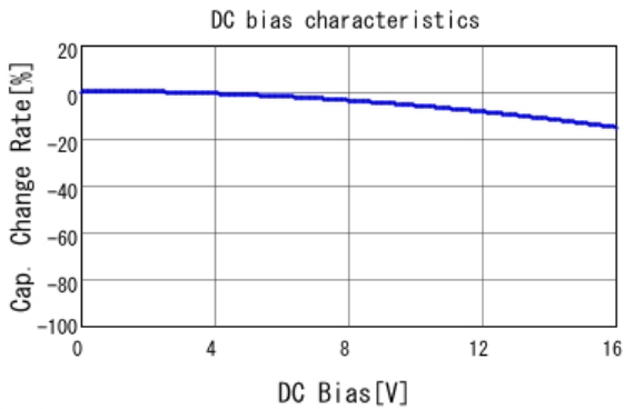
■ GCM21BR71C474KA37 C-DC bias capchange, 25.0degC, AC1.
