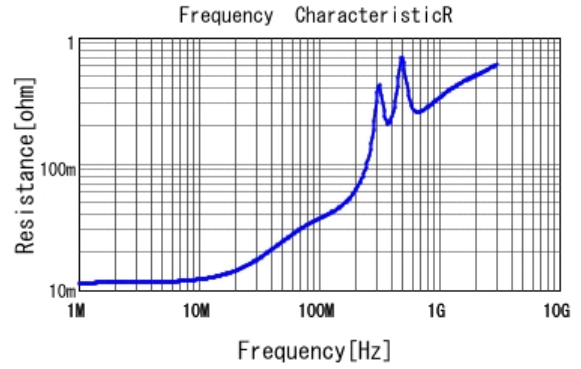
■ GCM21A7U2E222JX01 R DC0V, 25degC
