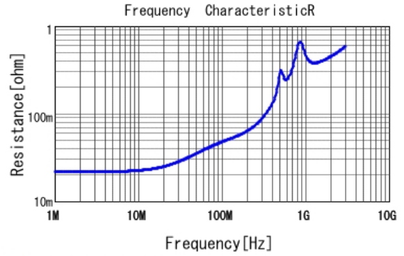
■ GCM21A7U2E122JX01 R DC0V, 25degC
