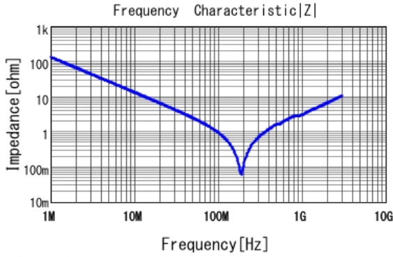
■ GCM21A7U2E122JX01 |Z| DC0V, 25degC
