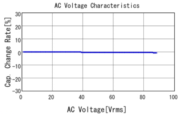
■ GCM21A7U2E122JX01 C-AC Voltage capchange, DC0V, 25.0d
