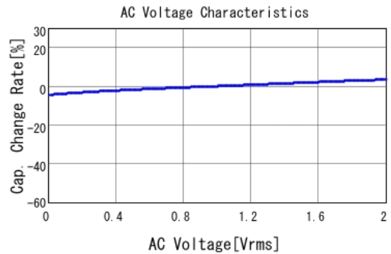
■ GCM219R71H334KA55 C-AC Voltage capchange, DCOV, 25.0d
