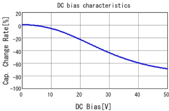
■ GCM219R71H334KA55 C-DC bias capchange, 25.0degC, AC1.
