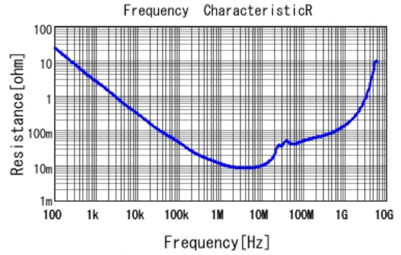
■ GCM219R71H334KA55 R DCOV, 25degC
