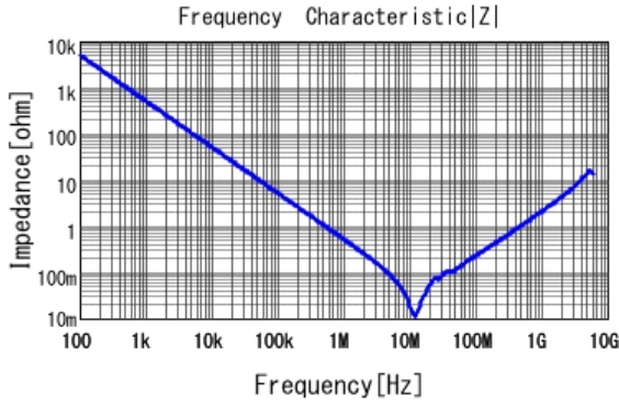
■ GCM219R71H334KA55 |Z| DCOV, 25degC
