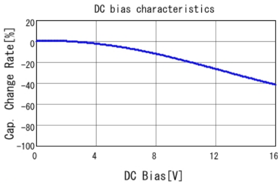
GCM219R71C684KA37 C-DC bias capchange, 25.0degC, AC1.
