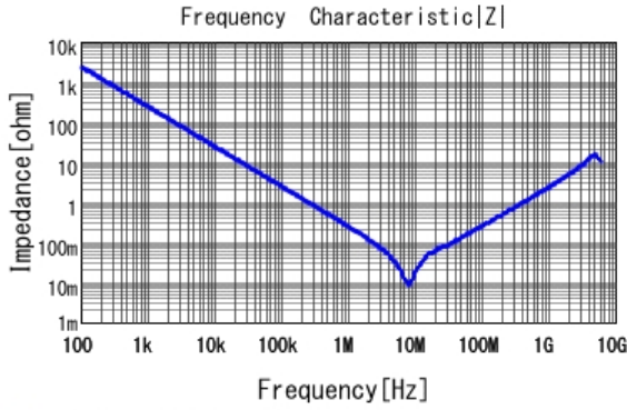
GCM219R71C684KA37 |Z| DCOV, 25degC
