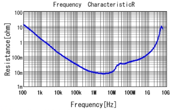
GCM219R71C684KA37 R DCOV, 25degC
