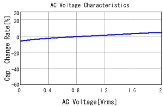
GCM219R71C684KA37 C-AC Voltage capchange, DCOV, 25.0d
