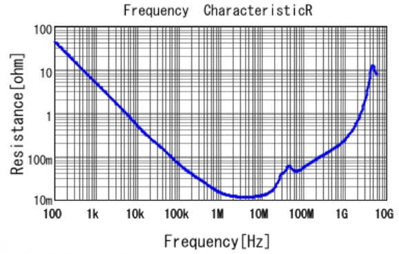
■ GCM219R71C224KA37 R DC0V, 25degC
