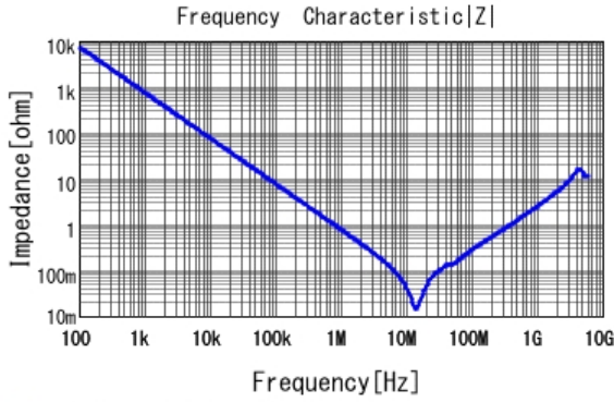
■ GCM219R71C224KA37 |Z| DC0V, 25degC
