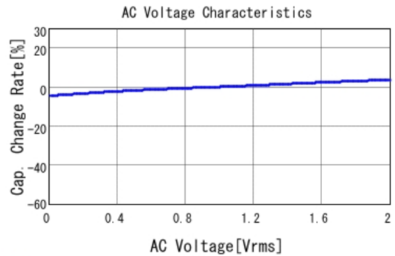
■ GCM219R71C224KA37 C-AC Voltage capchange, DC0V, 25.0d
