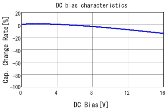
■ GCM219R71C224KA37 C-DC bias capchange, 25.0degC, AC1.
