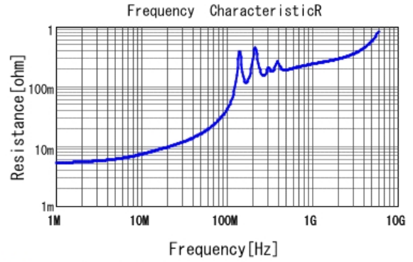
■ GCM2195C1K103JA16 R DCOV, 25degC
