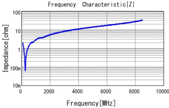
■ GCM2165C2A681JA16 |Z| DC0V, 25degC
