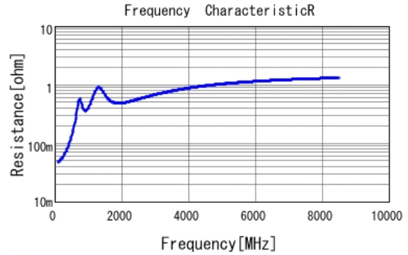
■ GCM2165C2A681JA16 R DC0V, 25degC
