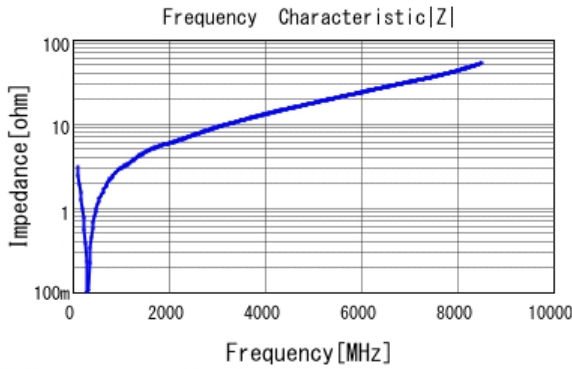
■ GCM2165C2A471JA16 |Z| DC0V, 25degC
