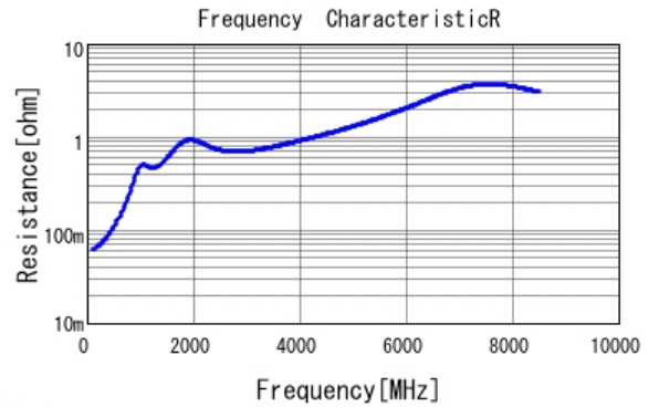
■ GCM2165C2A471JA16 R DC0V, 25degC
