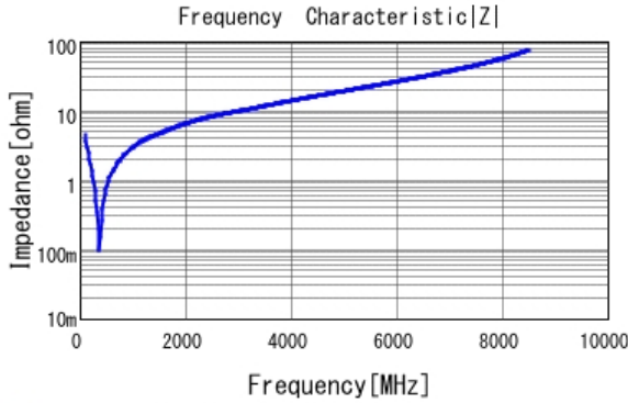
■ GCM2165C2A331JA16 |Z| DCOV, 25degC
