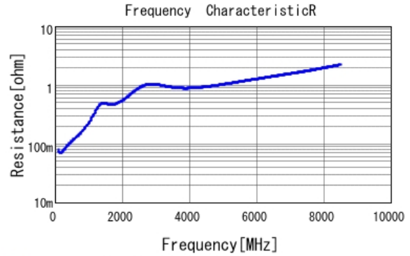
■ GCM2165C2A331JA16 R DCOV, 25degC
