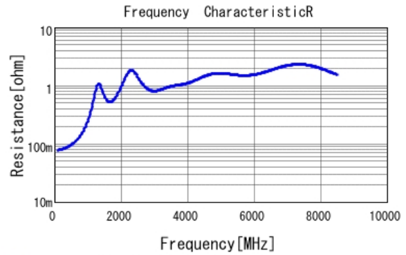
■ GCM2165C2A221JA16 R DC0V, 25degC
