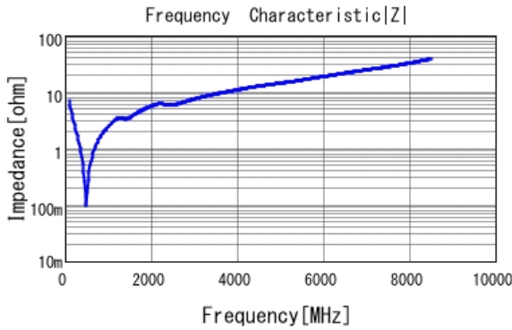
■ GCM2165C2A221JA16 |Z| DC0V, 25degC
