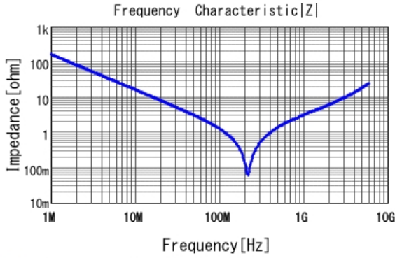
■ GCM2165C2A102JA16 |Z| DCOV, 25degC
