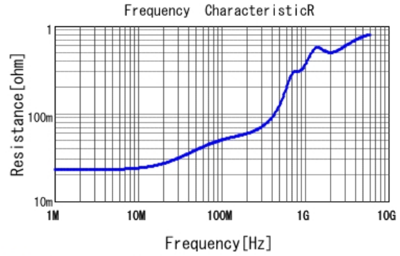
■ GCM2165C2A102JA16 R DCOV, 25degC
