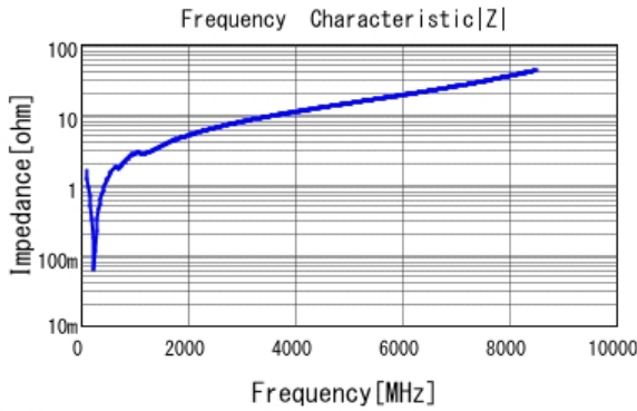
■ GCM2165C1H821JA16 |Z| DCOV, 25degC
