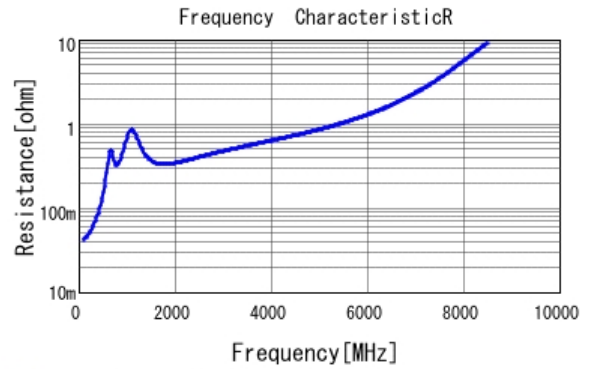
■ GCM2165C1H821JA16 R DCOV, 25degC
