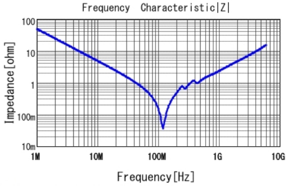
■ GCM2165C1H332JA16 |Z| DCOV, 25degC
