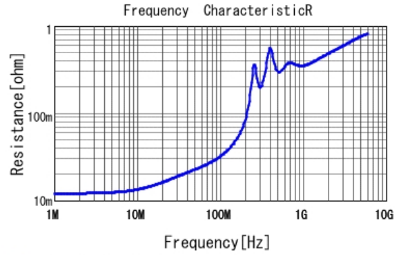
■ GCM2165C1H332JA16 R DCOV, 25degC
