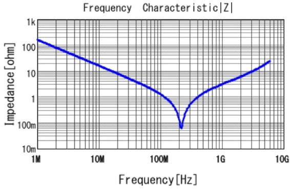
■ GCM2165C1H102JA16 |Z| DCOV, 25degC
