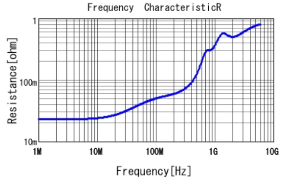
■ GCM2165C1H102JA16 R DCOV, 25degC
