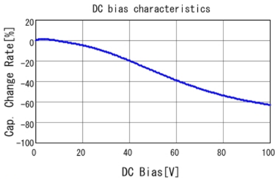
GCM188R72A153KA37 C-DC bias capchange, 25.0degC, AC1.
