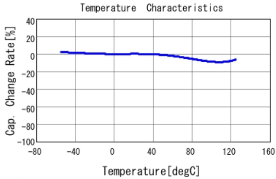
■ GCM188R72A153KA37 C-Temp. capchange, DC0.0V, AC1.0V rm
