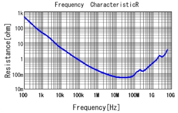
GCM188R72A153KA37 R DC0V, 25degC
