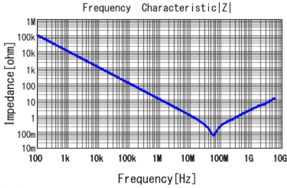
GCM188R72A153KA37 |Z| DC0V, 25degC
