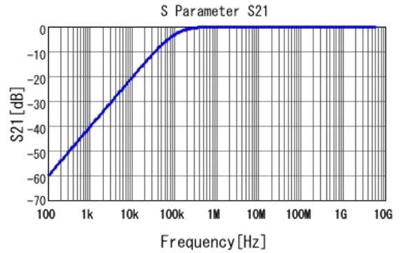
■ GCM188R72A153KA37 S21 DC0V, 25degC
