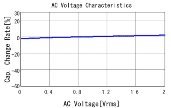
GCM188R72A153KA37 C-AC Voltage capchange, DC0V, 25.0d
