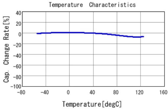
■ GCM188R71H683KA57 C-Temp. capchange, DC0.0V, AC1.0Vrms
