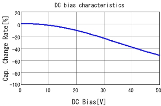
GCM188R71H683KA57 C-DC bias capchange, 25.0degC, AC1.
