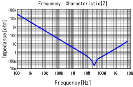
GCM188R71H683KA57 |Z| DCOV, 25degC
