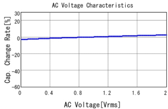
GCM188R71H683KA57 C-AC Voltage capchange, DCOV, 25.0d
