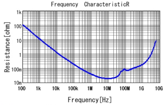
GCM188R71H683KA57 R DCOV, 25degC
