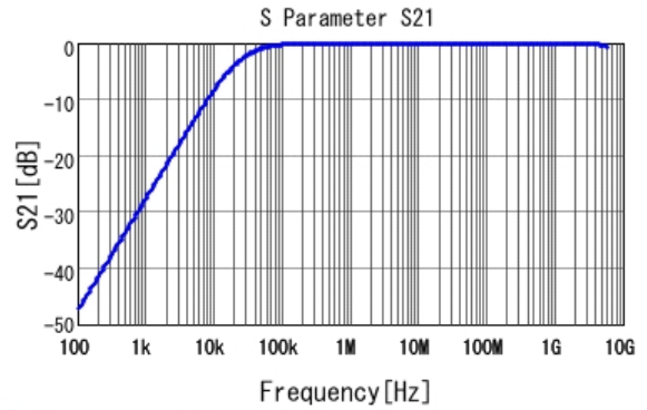
■ GCM188R71H683KA57 S21 DC0V, 25degC
