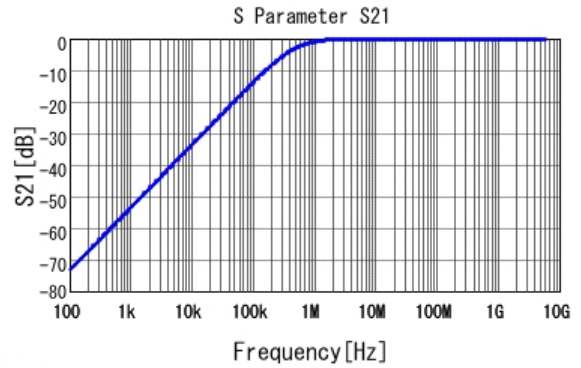
■ GCM188R71H332KA37 S21 DC0V, 25degC
