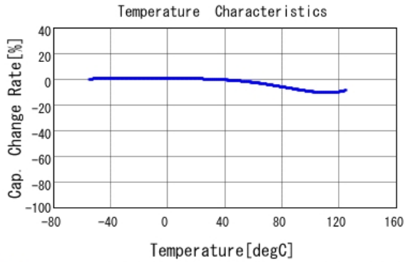
■ GCM188R71H332KA37 C-Temp. capchange, DC0.0V, AC1.0V rm
