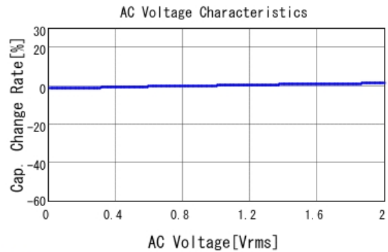
GCM188R71H152KA37 C-AC Voltage capchange, DCOV, 25.0d
