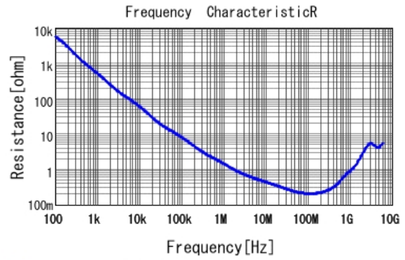
GCM188R71H152KA37 R DCOV, 25degC
