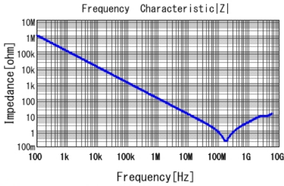
GCM188R71H152KA37 |Z| DCOV, 25degC
