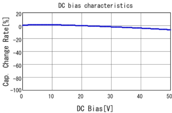
GCM188R71H152KA37 C-DC bias capchange, 25.0degC, AC1.
