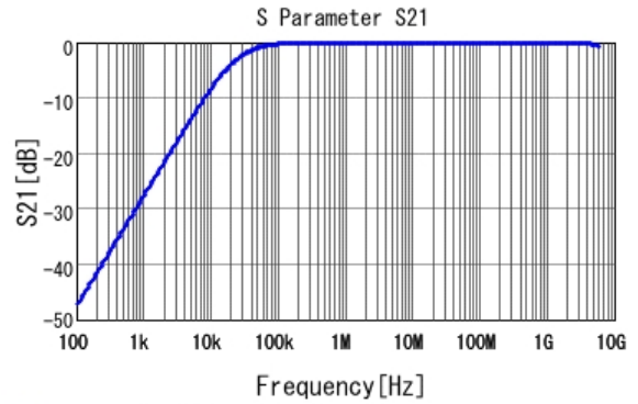
■ GCM188R71E683KA57 S21 DC0V, 25degC
