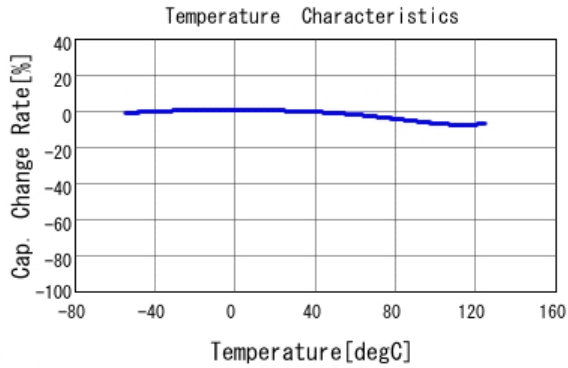
■ GCM188R71E683KA57 C-Temp. capchange, DC0.0V, AC1.0Vrm
