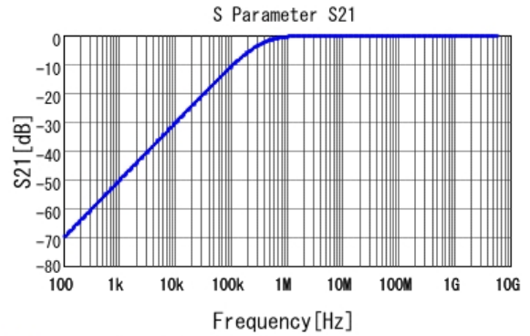
■ GCM188R71E472KA37 S21 DC0V, 25degC
