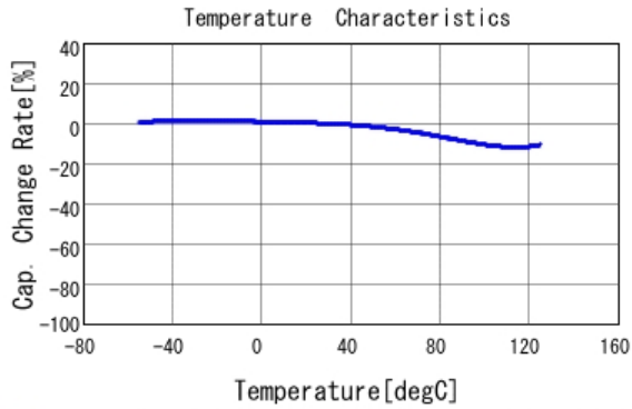
■ GCM188R71E472KA37 C-Temp. capchange, DC0.0V, AC1.0Vrm
