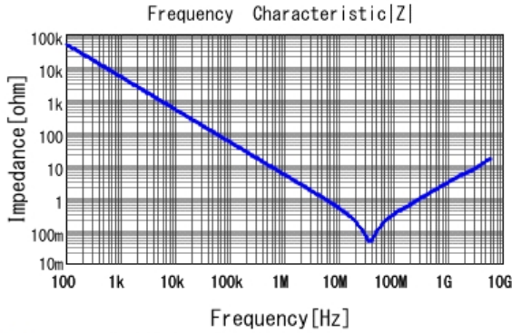
GCM188R71E333KA37 |Z| DCOV, 25degC
