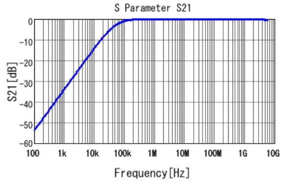
■ GCM188R71E333KA37 S21 DC0V, 25degC
