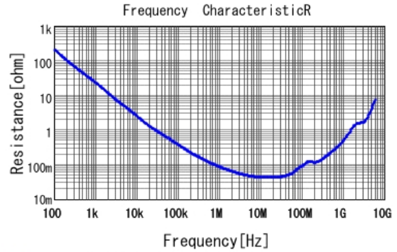
GCM188R71E333KA37 R DCOV, 25degC
