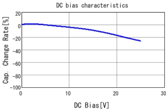
GCM188R71E333KA37 C-DC bias capchange, 25.0degC, AC1.
