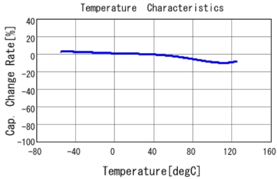
■ GCM188R71E333KA37 C-Temp. capchange, DC0.0V, AC1.0V rm
