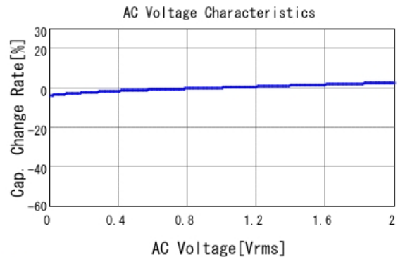
GCM188R71E333KA37 C-AC Voltage capchange, DCOV, 25.0d
