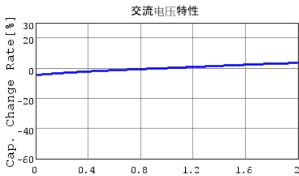
GCM188R71E224KA55 C-AC Voltage capchange, DC
