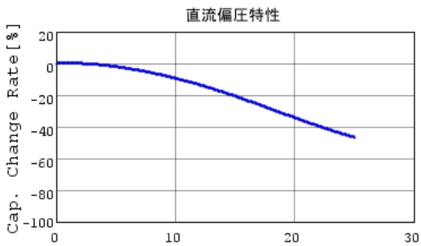
GCM188R71E224KA55 C-DC bias capchange, 25.0c
