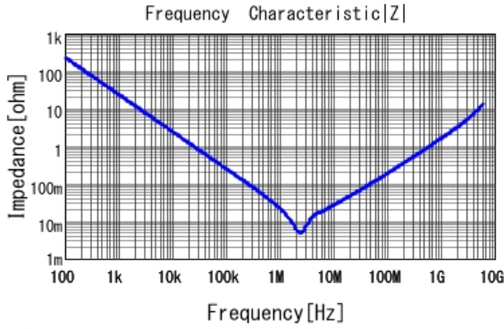
GCM188D70J106ME36 |Z| DCOV, 25degC
