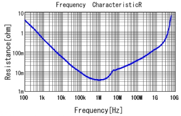
GCM188D70J106ME36 R DCOV, 25degC
