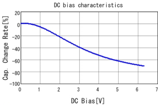
GCM188D70J106ME36 C-DC bias capchange, 25.0degC, AC1V
