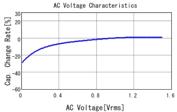
GCM188D70J106ME36 C-AC Voltage capchange, DCOV, 25.0d
